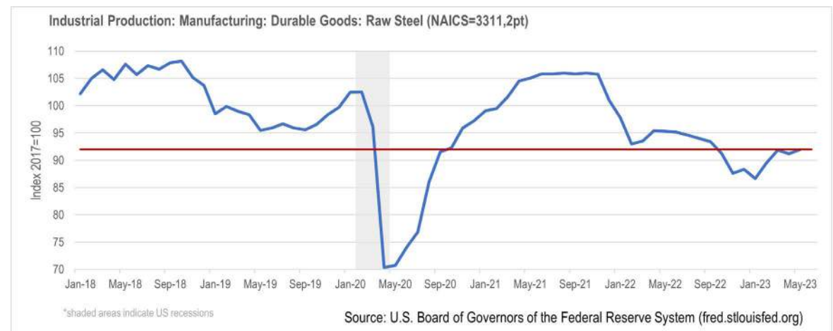
CHART 2: STEEL PRODUCTION
